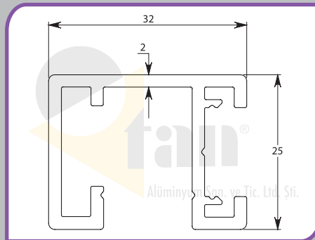
Profil 10-0008 Profile 10-0008 مقطع 10-0008
